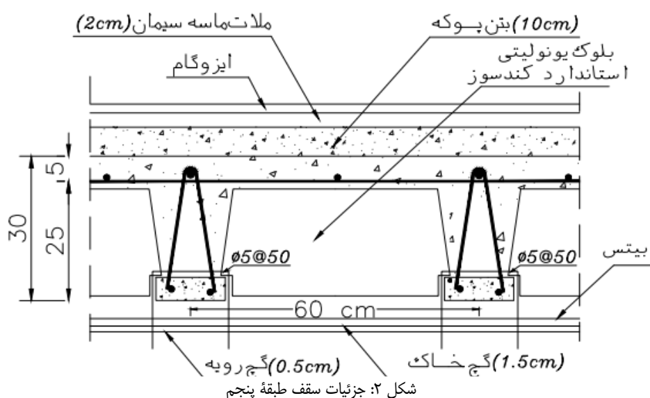
Fig 2: Roof details of the fifth floor
